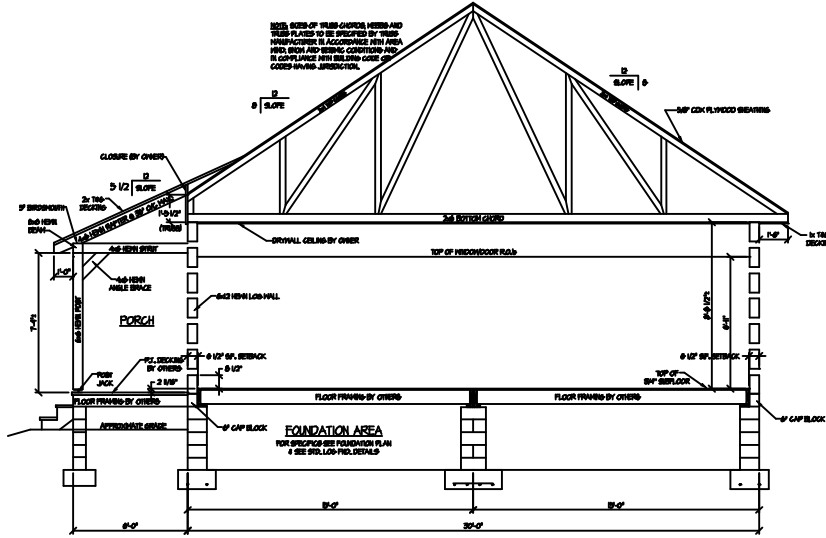
SECTION THRU BEDROOM/BATH/REAR PORCH
