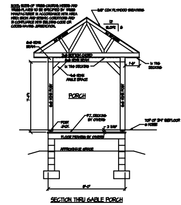
SECTION THRU GABLE PORCH
