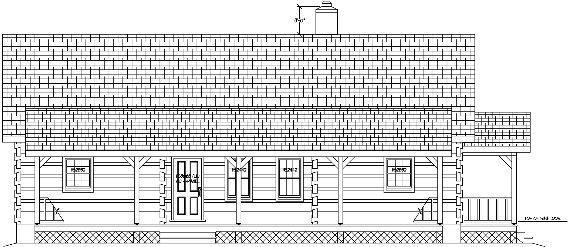
PLAN FRONT
