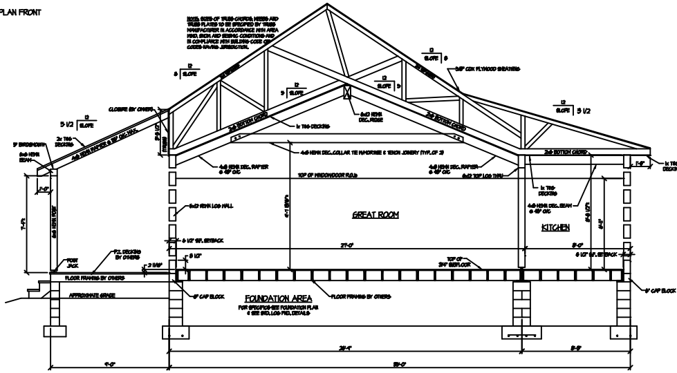
SECTION THRU GREAT ROOM/KITCHEN
