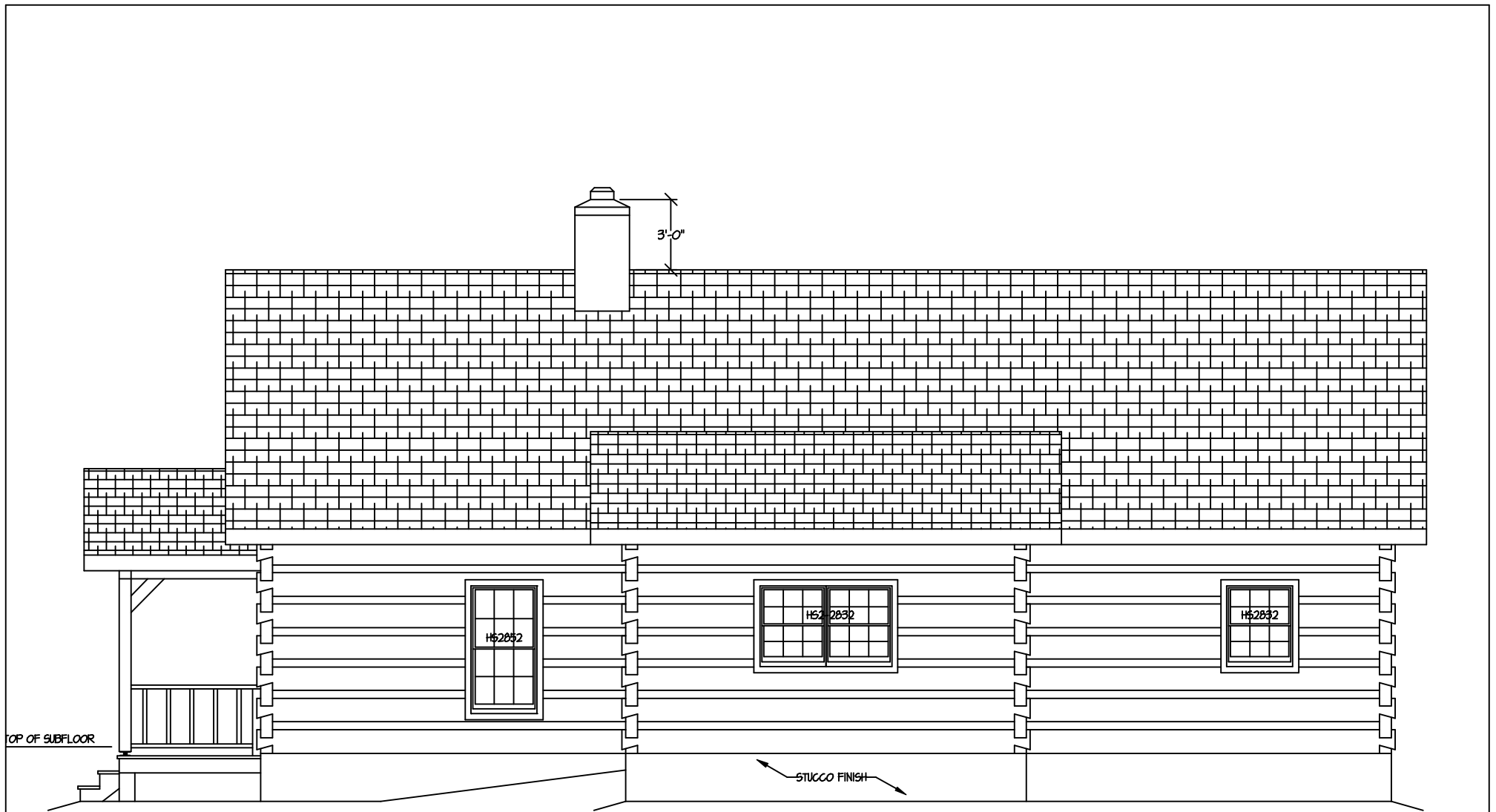
PLAN BACK
