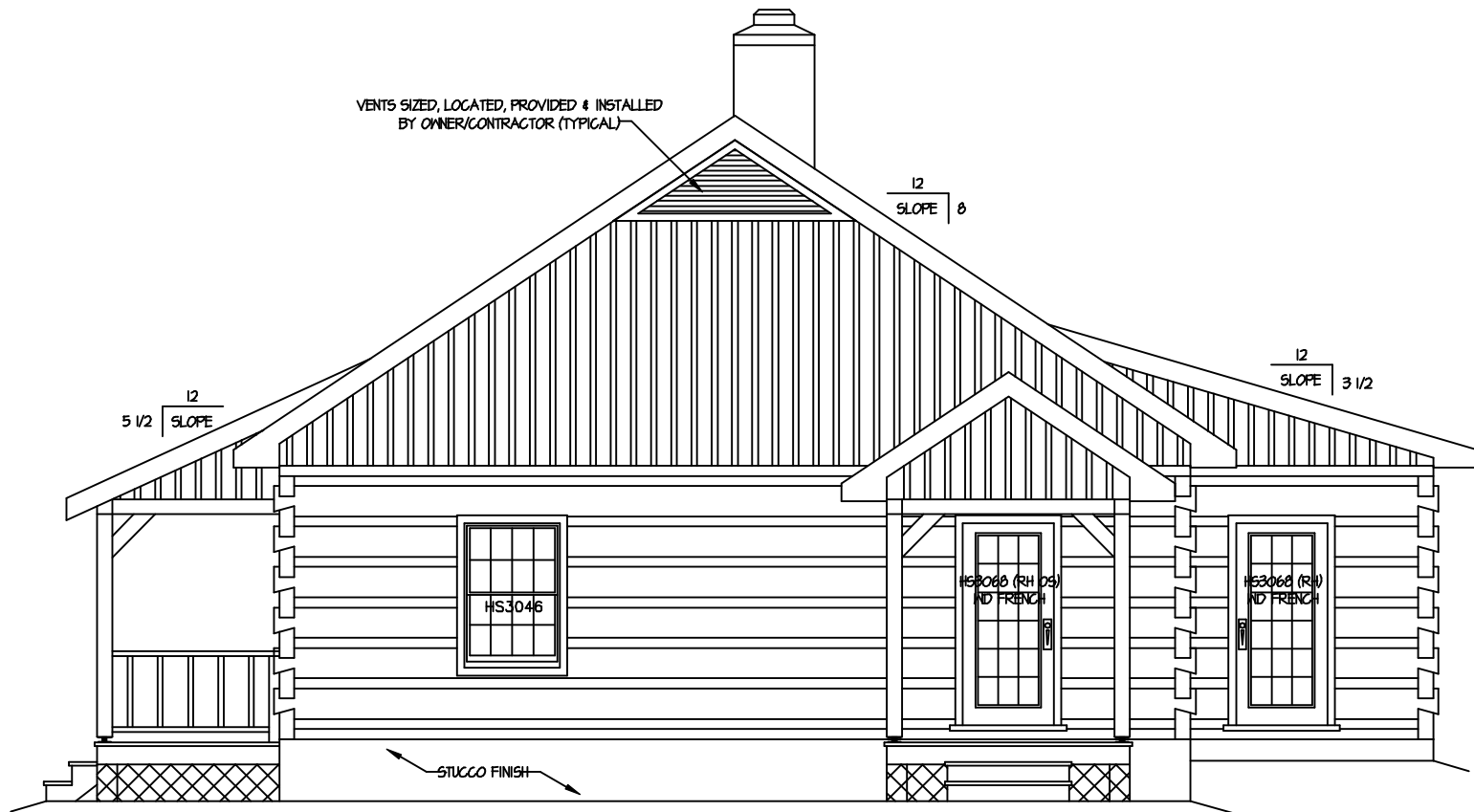
PLAN RIGHT
