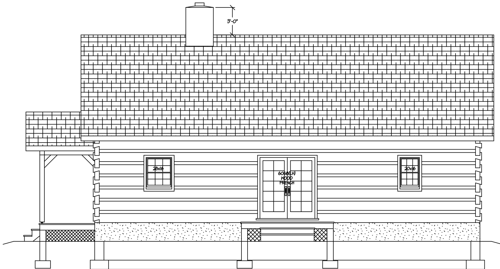
PLAN BACK
